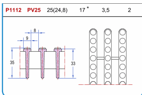
P1112 Mod. PV/25 rollable grating; mm. 250 x mm. 35
