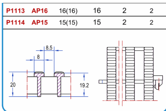
P1113 Mod. AP/16 rollable grating; fixed width mm. 160; fixed thickness mm. 20
