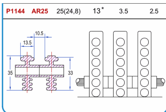
P1144 Mod. AR/25 rollable grating; mm 250 x mm 35
